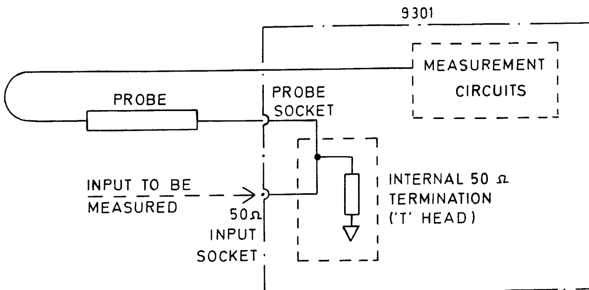
Probe And Input Connections For Internal 50Ω Termination
